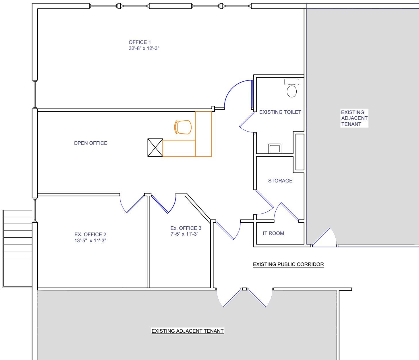
KEY PLAN: SECOND FLOOR
